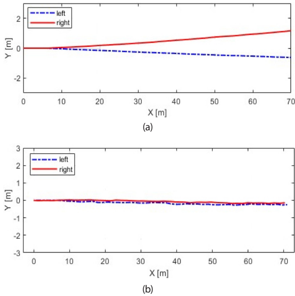
Fig. 6. Estimated position using each algorithm (straight trajectory). (a) standalone PDR. (b) proposed DF-PDR system.
