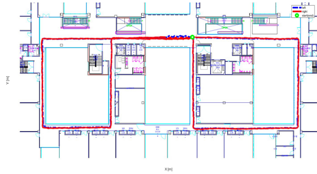
Fig. 9. Estimated position using proposed DF-PDR system.
