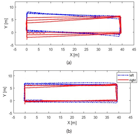
Fig. 8. Estimated position using each algorithm (square trajectory). (a) standalone PDR. (b) proposed DF-PDR system.
