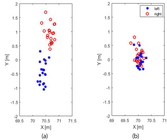
Fig. 7. Estimated positions at last step shoe. (a) standalone PDR. (b) proposed DF-PDR system.
