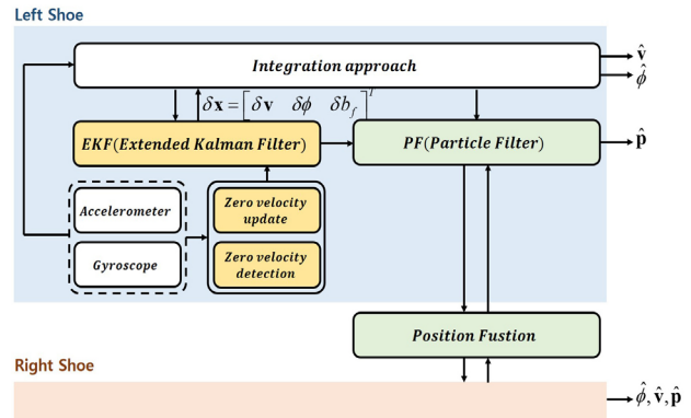
Fig. 3. Overall diagram of proposed method.
