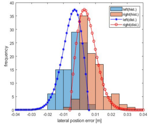
Fig. 2. Distribution of the lateral position error in one step.
