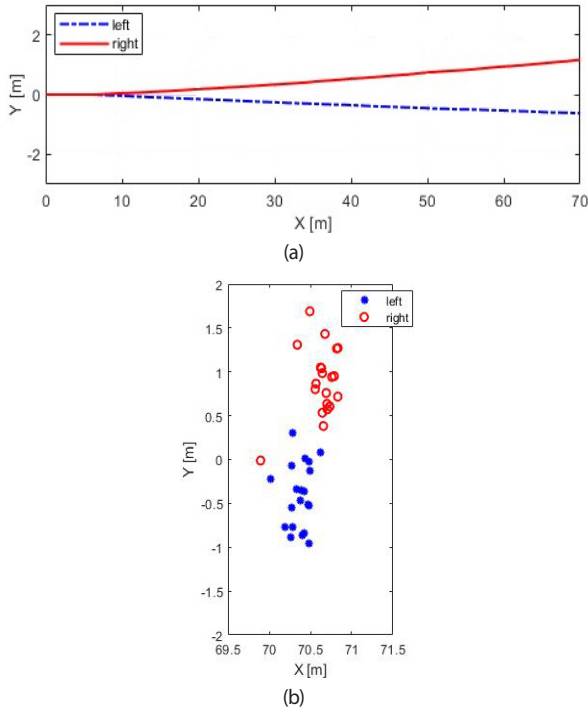
Fig. 1. Experimental results with each shoe. (a) average of estimated position with each shoe, (b) estimated positions at last step.
