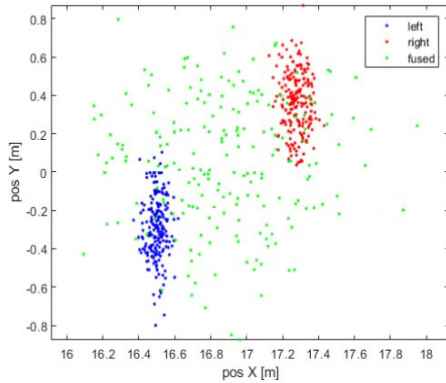
Fig. 4. Fused position represents the pedestrian's center.
