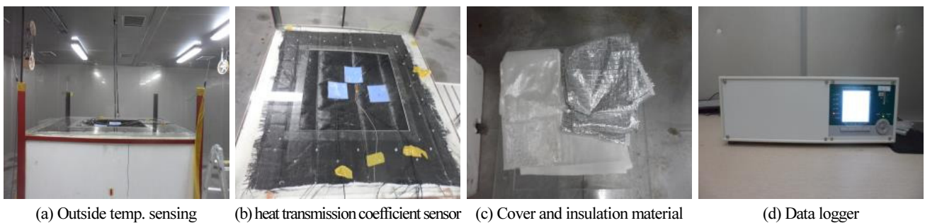
Fig. 2. Overall heat transmission coefficient measuring processes ((a), (b), (c), (d)).
