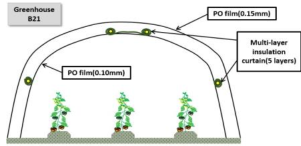
Fig. 4. A cover and an insulation curtain in PO film(B21).
