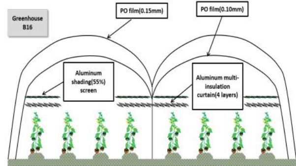
Fig. 6. A cover and an insulation curtain in PO film(B16).
