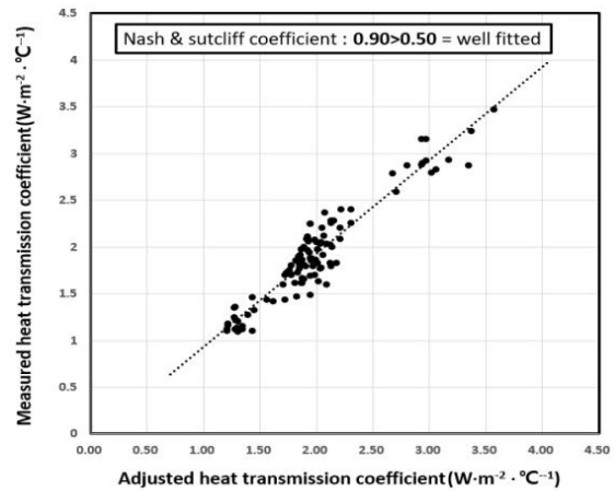
Fig. 8. Model estimated and measured heat transmission coefficients comparison diagram (1:1 equivalent line comparison) when installing multi-layers of cover and insulation material.
