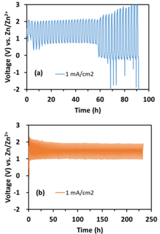
Fig. 10. Galvanostatic cell test in 1.0 M ZnSO 4 + 0.05 M H 2 SO 4 as electrolyte. (a) Zn/PtRu, and (b) Zn/MnO 2
