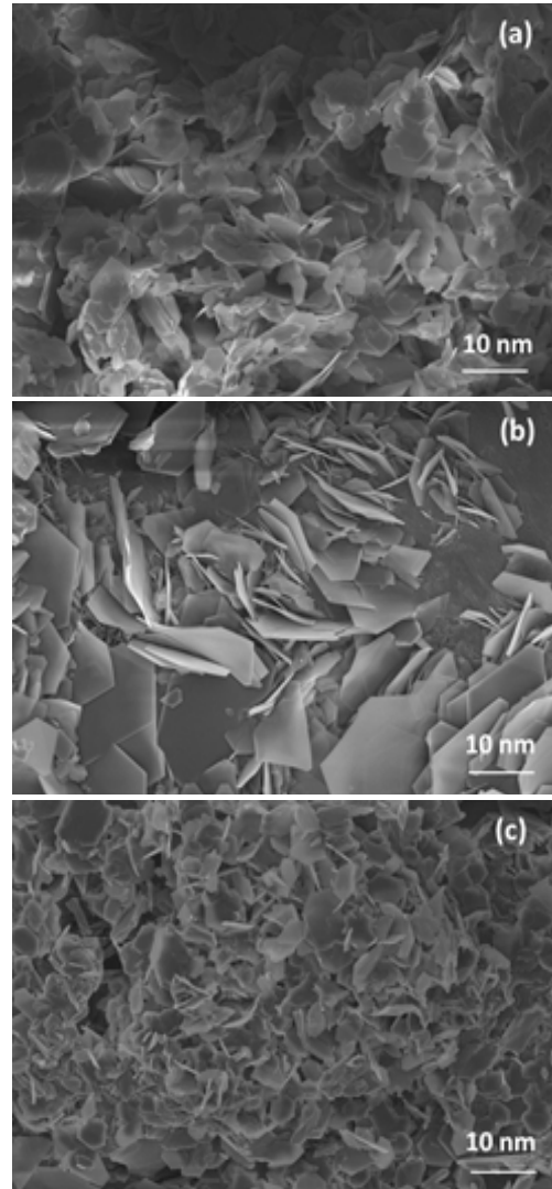
Fig. 6. SEM images of the Zn after 100 plating/stripping cycles in different electrolytes. (a) 1.0 M ZnSO 4 + 0.05 M H 2 SO 4 , (b) 1.0 M ZnSO 4 + 0.005 M H 2 SO 4 , (c) 1.0 M ZnSO 4 + 0.0005 M H 2 SO 4
