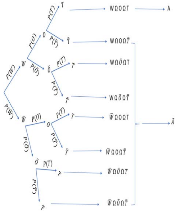
Fig. 7. Probability of activating a session using a weighted tree
