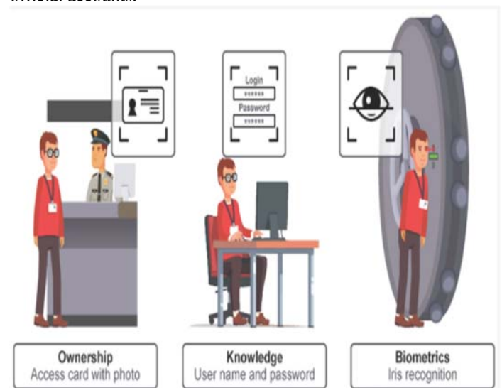
Fig. 1 Authentication methods [5]
