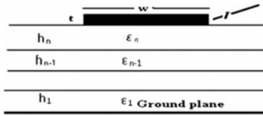
Fig2: microstrip multilayer antenna permittivity
