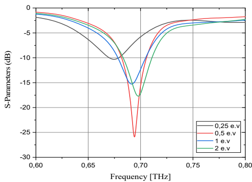
Fig5 Graphene-microstrip patch antenna return loss adjustment vs Fermi level value E_F .
