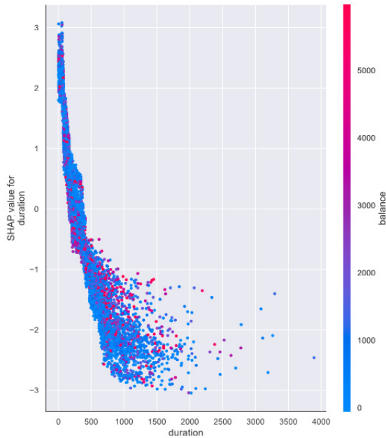
〈Figure 6〉 SHAP Dependent Plot Shows that Effect of Duration on Model Output with Respect to Balance
