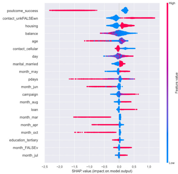
(Figure 8) Summary Plot of Selected SHAP Values on the Dataset Excluding Duration
