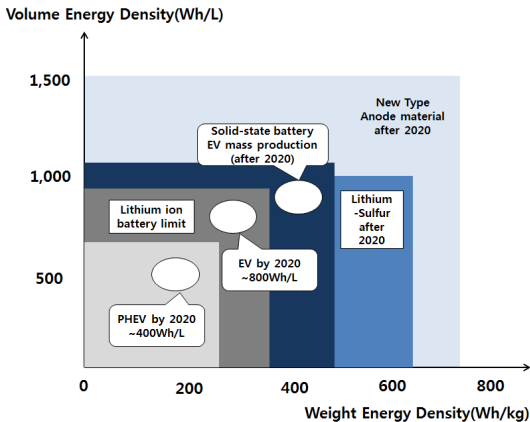
Fig. 1. Bosch's battery technology prospect 1)
