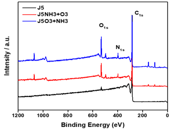
Fig. 1. XPS survey spectra of J5, J5NH3+O3 and J5O3+NH3
