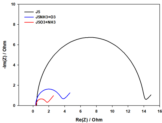
Fig. 3. Nyquist plots of J5, J5NH3+O3 and J5O3+NH3 graphite felts in a frequency range from 10^{-2} to 10^5 Hz in 0.1 M \text{VOSO}_4 +3.0 M \text{H}_2\text{SO}_4 electrolyte at open circuit voltage
