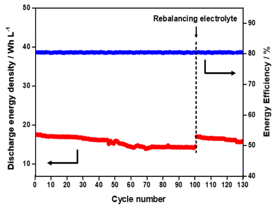
Fig. 6. The discharge energy density and energy efficiency of the J5O3+NH3 according to the number of cycles at 100 \text{ mA/cm}^2
