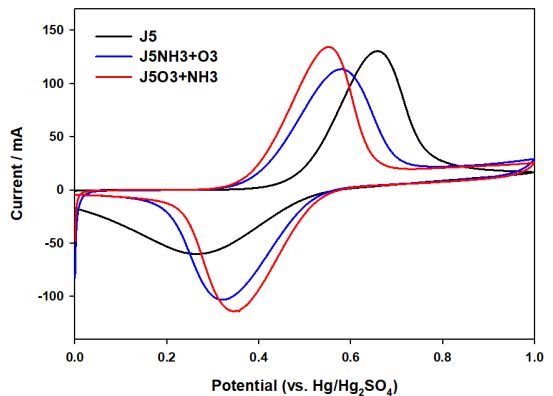
Fig. 2. Cyclic voltammograms of J5, J5NH3+O3 and J5O3+NH3 graphite felts with 0.1 M VOSO 4 +3.0 M H 2 SO 4 electrolyte at a scan rate of 5 mV/s with potential window of 0.0 V to 1.0 V vs. Hg/Hg 2 SO 4
