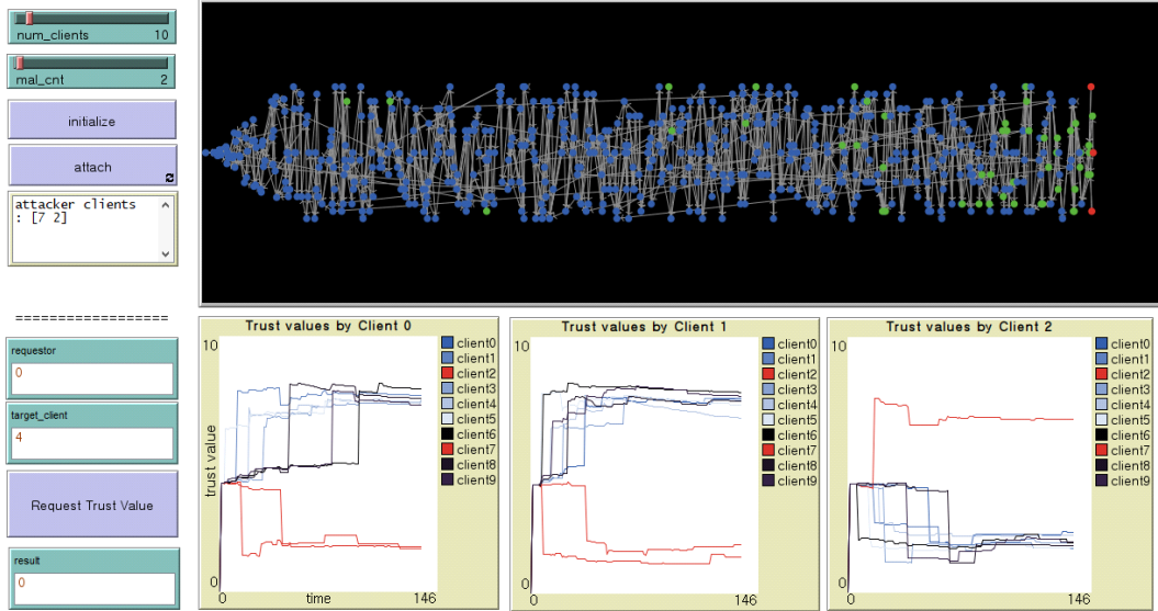
Fig. 5. Simulation GUI
