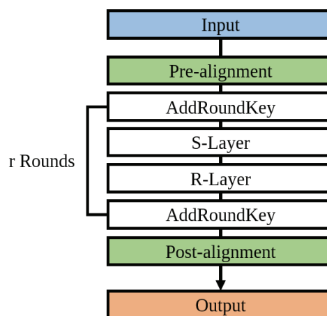
Fig. 6. Revised Algorithm Flow with Least Register-alignment
