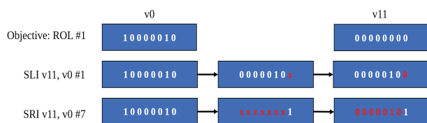
Fig. 5. Implement of Rotate Algorithm with Vector Instructions
