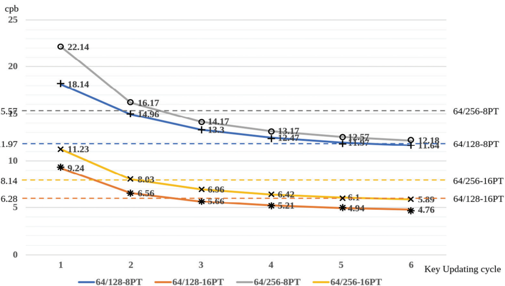
Fig. 7. Performance Measurement Graph
