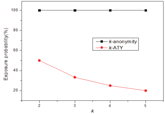
Fig. 4. User's Trajectory Exposure Probability
