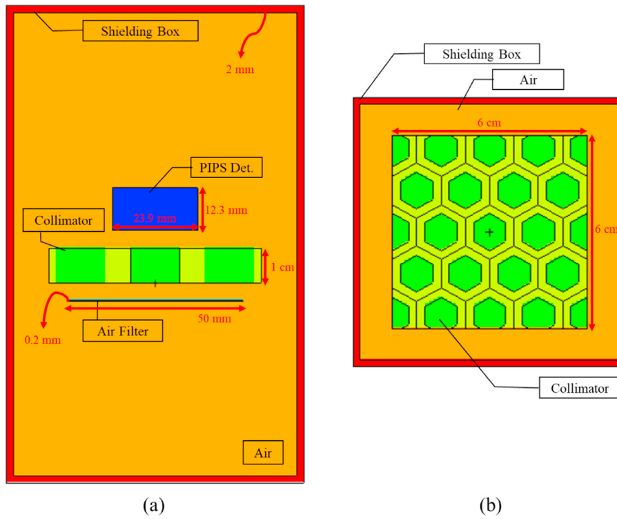
Fig. 2. Schematic representation of alpha detection system for simulation ((a) longitudinal section and (b) cross-section of the collimator).
