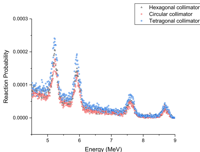
Fig. 6. Spectrum graph according to the shape of hole of collimator.
