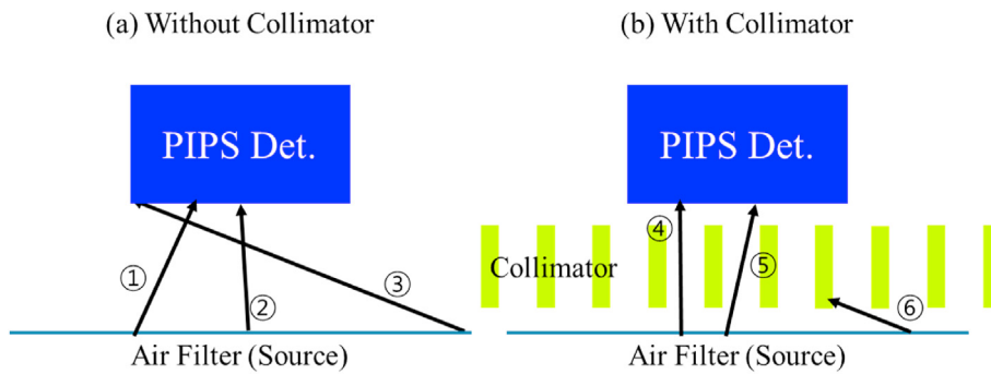
Fig. 3. Schematic representation of the incidence of alpha particles into PIPS detector, ((a) without collimator and (b) with collimator).
