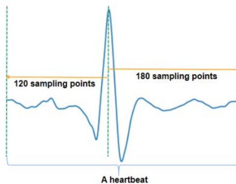
Fig. 4. Heartbeat segmentation.
