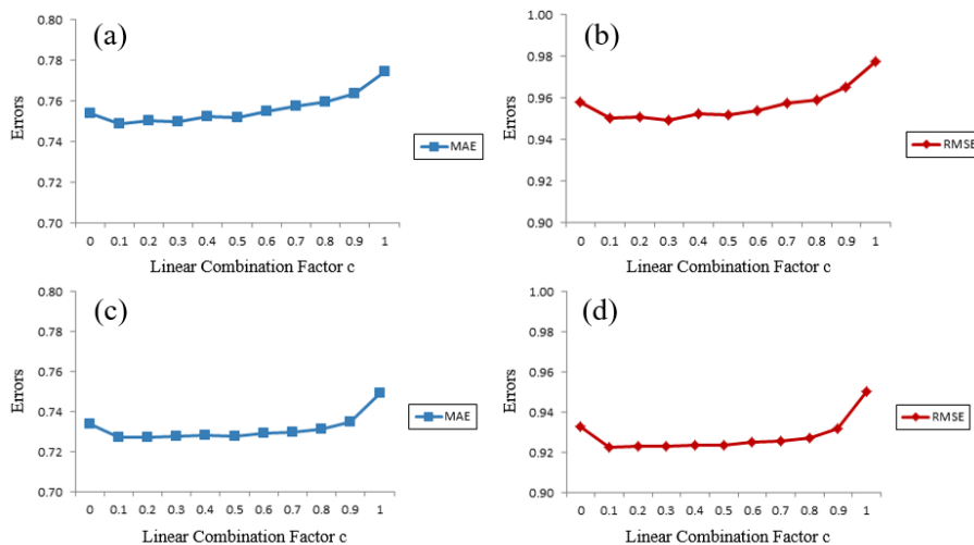
Fig. 3. Influence of linear combination factor c on the HCFCM-SL's prediction accuracy: (a) and (b) represents the results on the ml-100k dataset; (c) and (d) represents the results on the ml-1m dataset.
