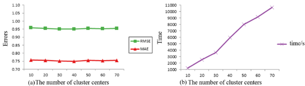
Fig. 2. Influence of the number of cluster centers on the HCFCM-SL algorithm.(a) Change of algorithm prediction accuracy with the number of cluster centers; (b) Change of algorithm running time with the number of cluster centers.
