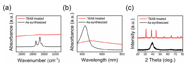
Fig. 2. As-synthesized TBAB-ligand-treated silver NC thin films: (a) FTIR data, (b) UV-vis data, and (c) X-ray diffraction (XRD) data.
