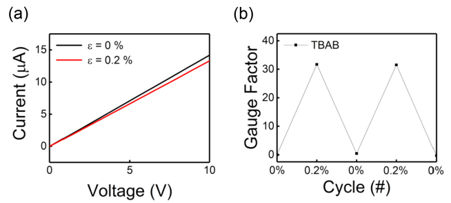
Fig. 5. TBAB-treated silver NC thin films on a 250 \mu\text{m} polyethylene terephthalate substrate strain sensor. (a) Electrical properties at 0% and 0.2% strain from 0 V to 10, (b) Bending test data at 0% to 0.2% strain at 10 V.
