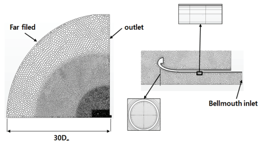
Fig. 4 Computational model.
