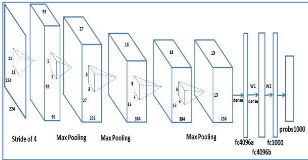
Fig. 1 AlexNet Architecture.
