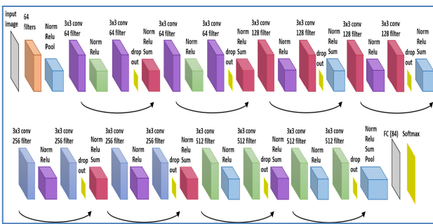
Fig. 2 ResNet18 Architecture.
