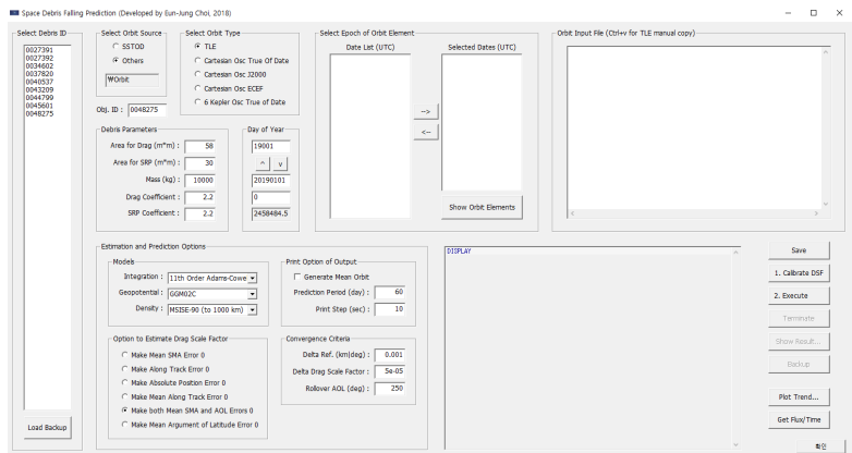
Fig. 1. SREP STEP 1. Select epoch of orbit element. SREP, Software for Re-Entry Prediction of space objects.
