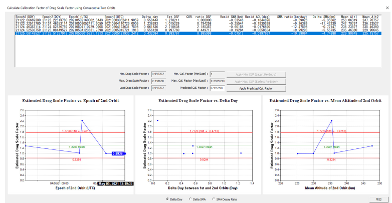
Fig. 2. SREP STEP 2. Estimate drag scale factor.
