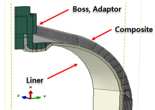
Fig. 2. Assembly of composite pressure vessel
