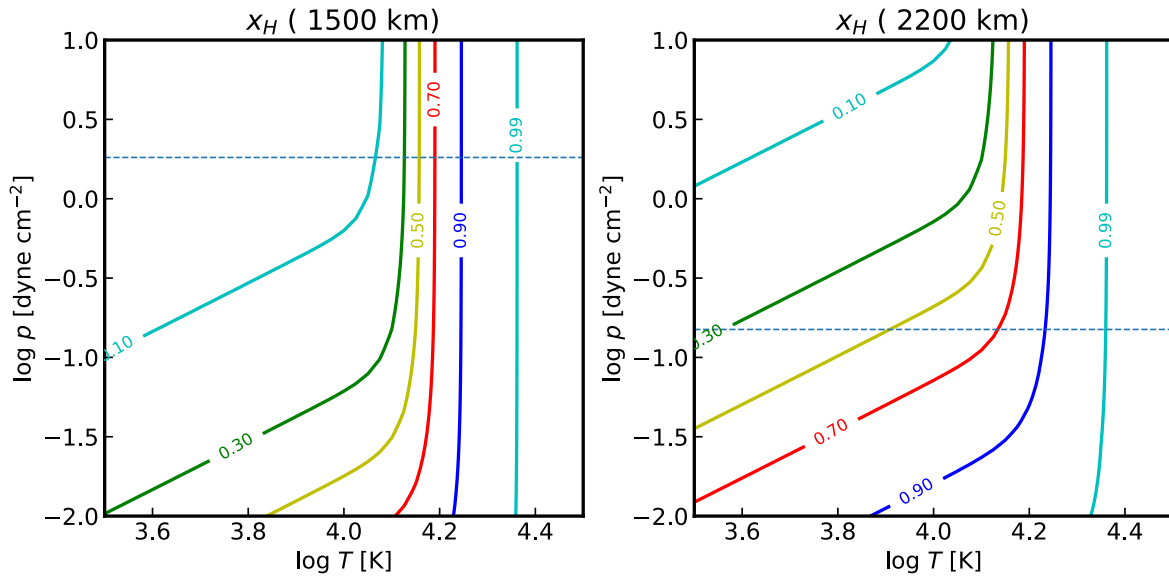
Fig. 5. Ionization degree of hydrogen of a plasma feature calculated using R_{ik} = 6.0 \times 10^{-4} \text{ s}^{-1} at 1,500 km (left) and using R_{ik} = 7.0 \times 10^{-3} \text{ s}^{-1} at 2,200 km (right), as obtained from the FALC model. The pressure value of the FALC model at the specified height is indicated by the dashed line in each plot for reference.
