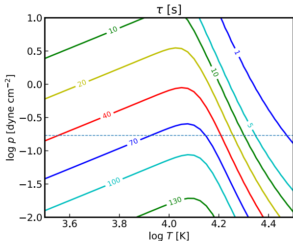
Fig. 6. Relaxation time for ionization equilibrium of a plasma feature in the upper chromosphere. The pressure value of the FALC model at 2,200 km is indicated by the dashed line for reference.
