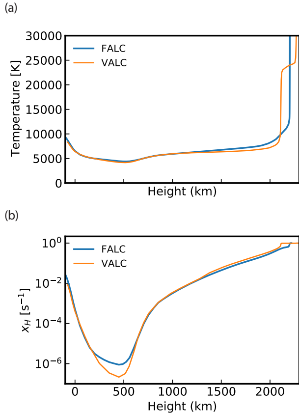
Fig. 2. Height variation of the temperature in the FALC model and VALC model (a), and ionization degree of hydrogen in the atmospheric models (b).
