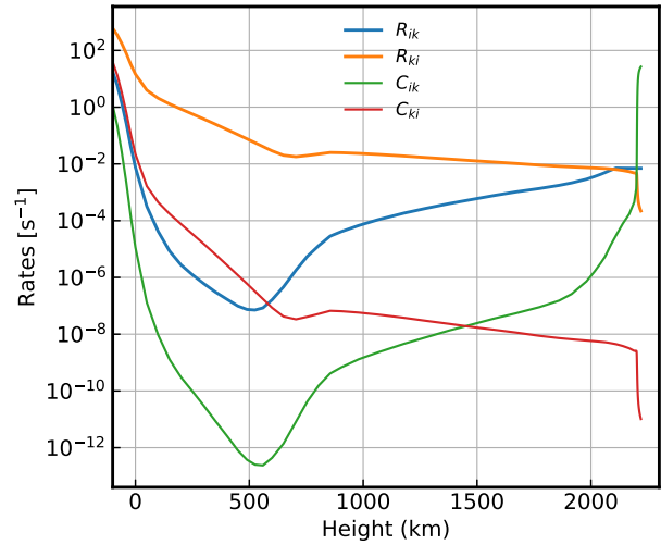
Fig. 3. Height variations of the transition rates in the FALC model.
