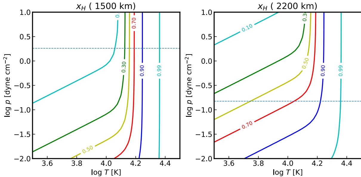
Fig. 7. Ionization degree of hydrogen of a plasma feature calculated using R_{ik} = 8.0 \times 10^{-4} \text{ s}^{-1} at 1,500 km (left) and using R_{ik} = 1.2 \times 10^{-2} \text{ s}^{-1} at 2,200 km (right) as obtained from the VALC model. The pressure value of the FALC model at the specified height is indicated by the dashed line in each plot for reference.
