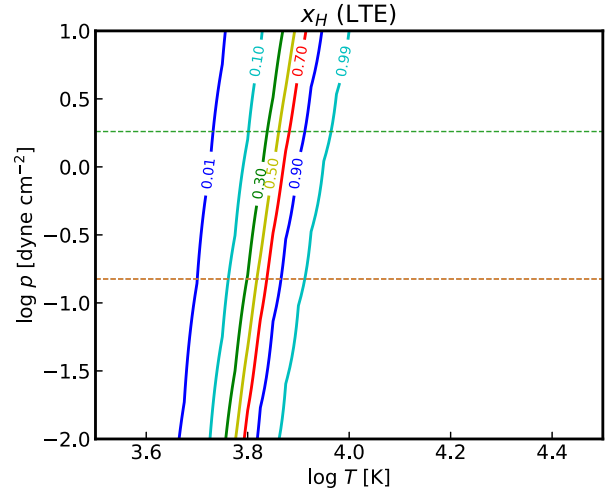
Fig. 4. Ionization degree of hydrogen of a plasma feature calculated in the LTE case. The two pressure values at heights of 1,500 km and 2,200 km are indicated by dashed lines for reference. LTE, local thermodynamic equilibrium.
