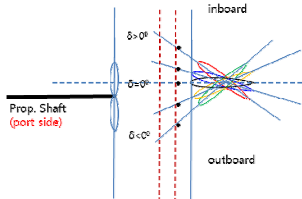
Fig. 5 Definition of rudder deflection angle
