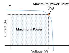
Fig. 2. Current-Voltage (IV) characteristic curve of solar cell
