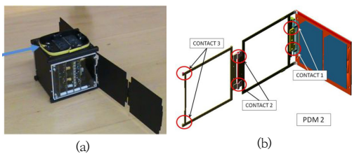
Fig. 4. Solar panel mechanism built into the project Xatcobero prototype and panel deployment mechanism simulation[12]
