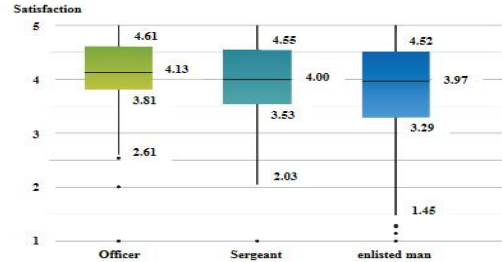
Fig. 5. Analysis of Variance result
