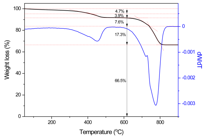
Figure 7. TGA thermogram of the asphalt pavement wear particles.
