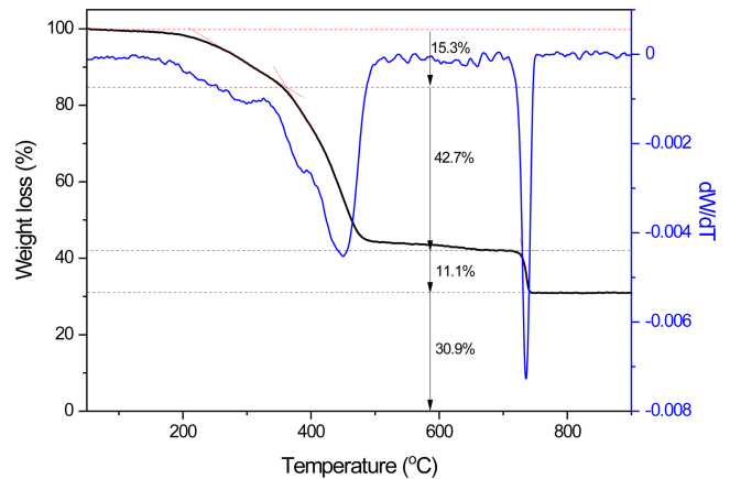
Figure 2. TGA thermogram of Sample 1.
