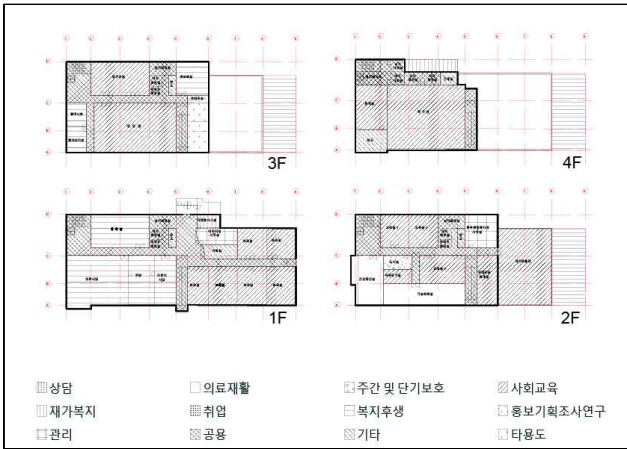
Fig. 6. Floor plans of Suncheon-dongbu SWC
