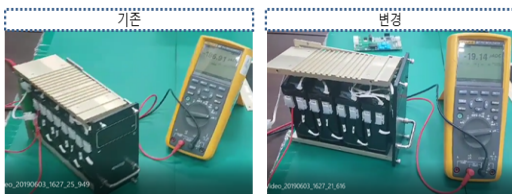
Fig. 22. Measured result of leakage current about Improved point in control board
