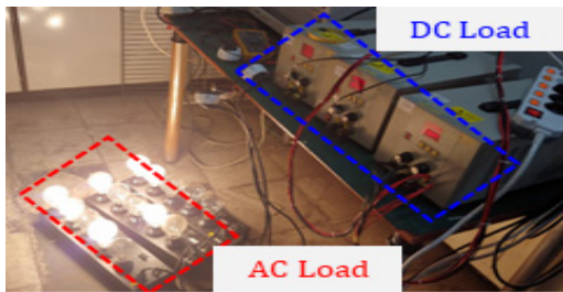
Fig. 25. ups test configuration of external temperature chamber
