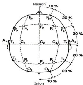
Fig. 3. Electrode locations of International 10-20 system for EEG recording
