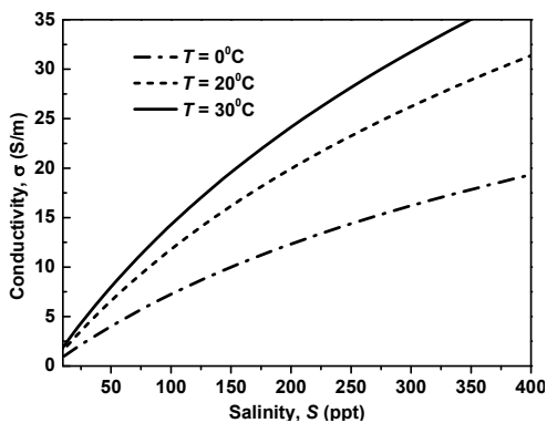
Fig. 2. Conductivity(σ) versus salinity(S) of salt-water at temperatures(T) (0, 20, 30 °C).
