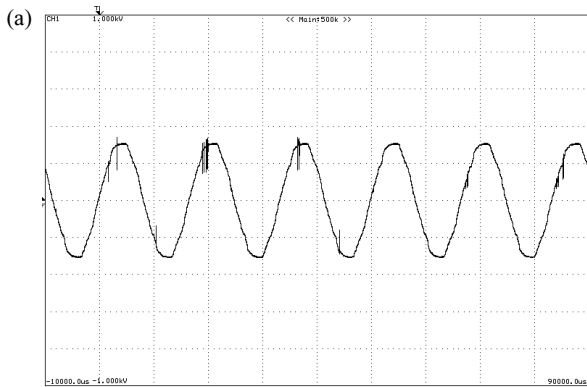
[200 V/div, 10ms/div]
