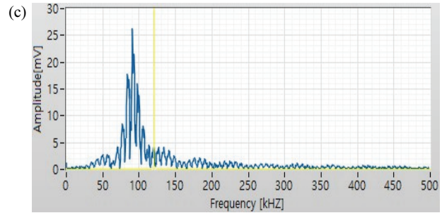
[5 mV/div, 100 kHz/div]
