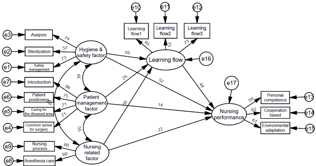
Fig. 1. Estimated parameters of the full latent structural equation model
