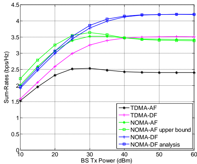
Fig. 6. Sum-rates under different BS power budgets
