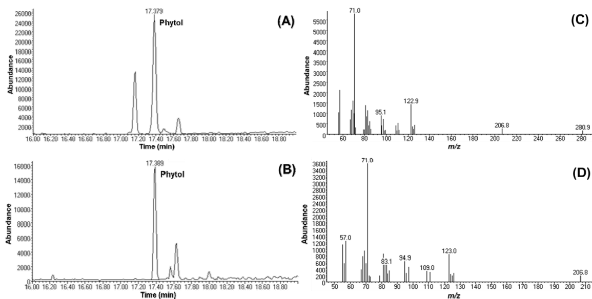
Fig. 5. GC-MS full scan ion monitoring chromatograms of (A) phytol and (B) HFSH, and the mass spectra of (C) phytol and (D) HFSH. GC-MS, gas chromatography-mass spectrometry; HFSH, n -hexane fraction of Schizophragma hydrangeoides .
