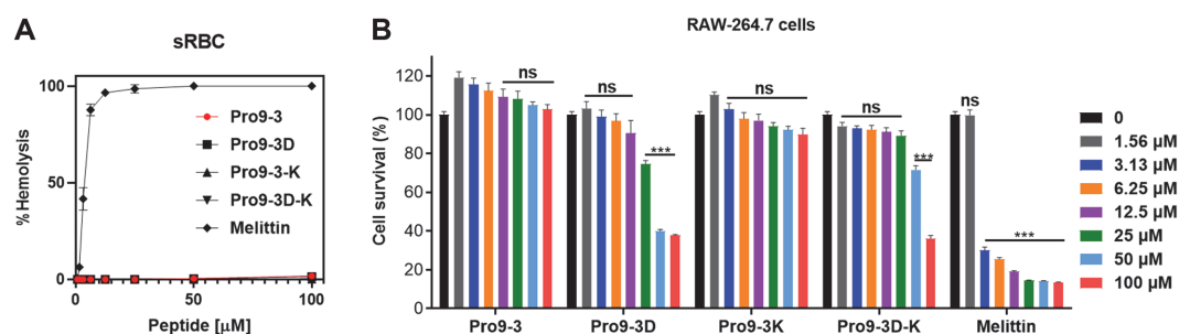
Fig. 1. Cytotoxicities of peptides. (A) Dose-dependent hemolytic activities in sheep red blood cell (sRBC) caused by peptides. (B) Dose-response cytotoxicities of the Pro9-3 and its analogs against RAW264.7 cells for 24 h. Melittin was used as a positive control. The values are expressed as the mean \pm SEM of three independent experiments: * p < 0.05 ; ** p < 0.01 ; *** p < 0.001 ; ns, not significant.
