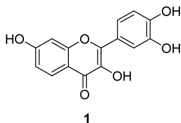
Figure 1. Chemical structure of fisetin.
