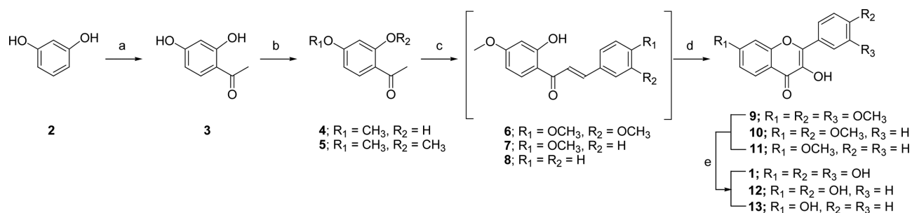
Scheme 1. Reagents and conditions: a) \text{Ac}_2\text{O} , \text{BF}_3\text{Et}_2\text{O} , E.A., 60^\circ\text{C} , 12 h, 95%; b) \text{Me}_2\text{SO}_4 , \text{K}_2\text{CO}_3 , Acetone, 60^\circ\text{C} , 7 h; c) substituted benzaldehyde, \text{KOH} , \text{MeOH} , 90^\circ\text{C} , 48 h; d) \text{NaOH} , \text{H}_2\text{O}_2 , r.t. 24 h, 42%; e) pyridine \text{HCl} , 160^\circ\text{C} , 12 h, 97%.
