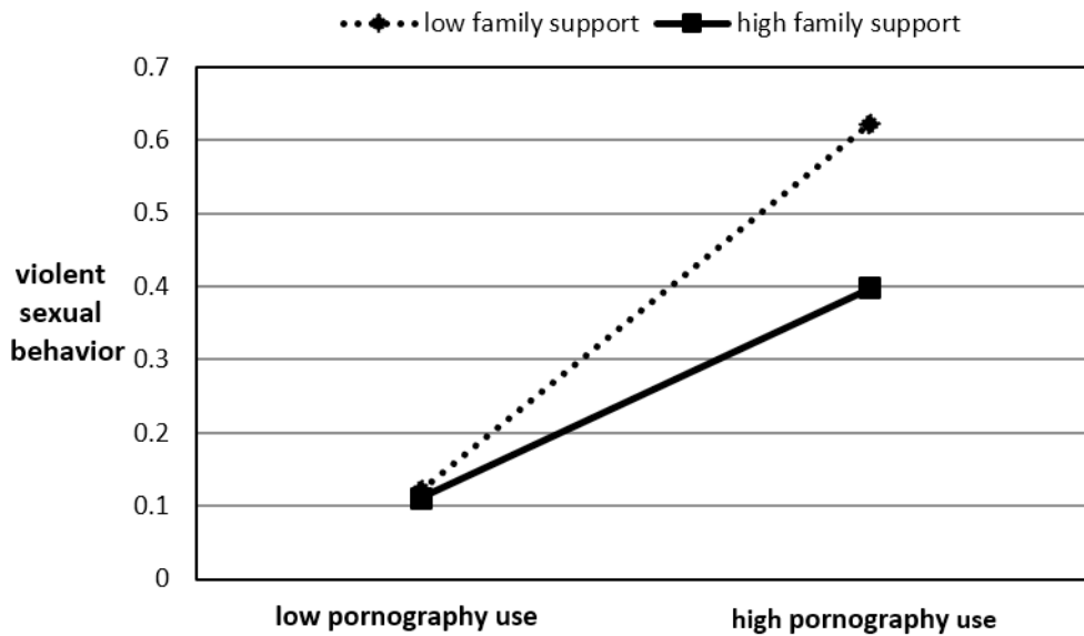
Figure 2. Interaction effect.
