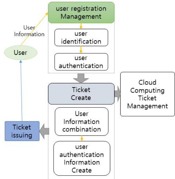
Fig. 5. Ticket Management
