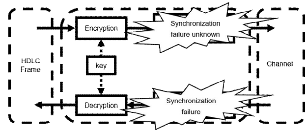
Fig. 1. CCSDS overall structure
