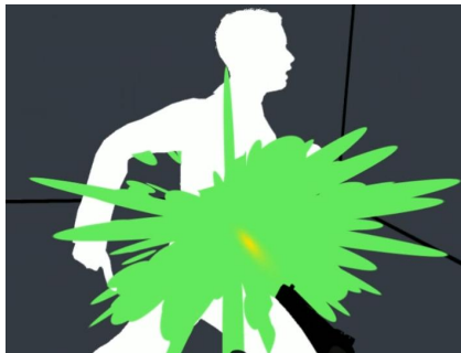
Fig. 9. Particle System
