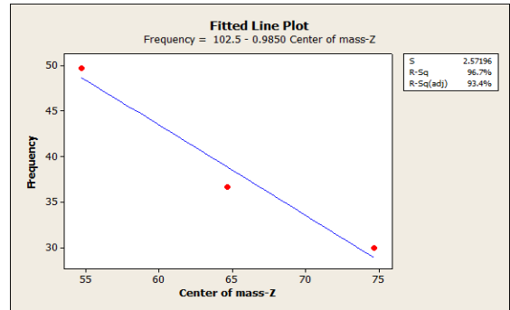
Fig. 12 Sensitivity analysis for design factors
