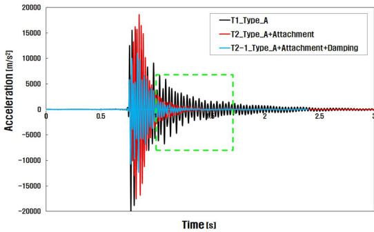
Fig. 6 Test result of type-A (time domain)
