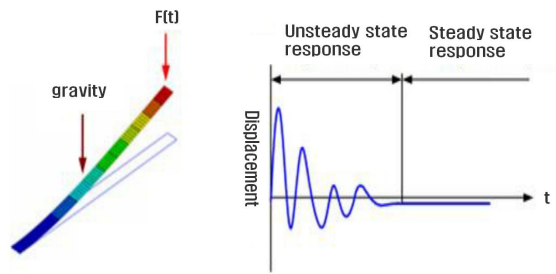
Fig. 2 Transient response of a cantilever beam
