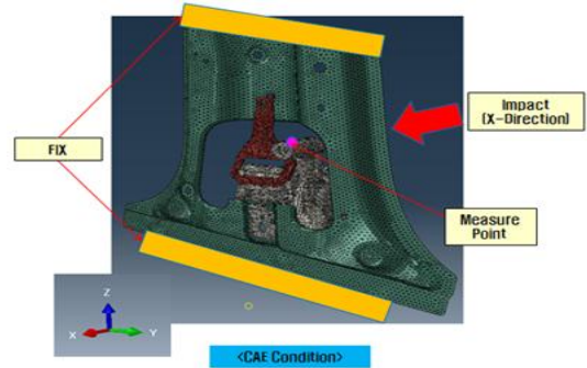
Fig. 8 Boundary condition for CAE
