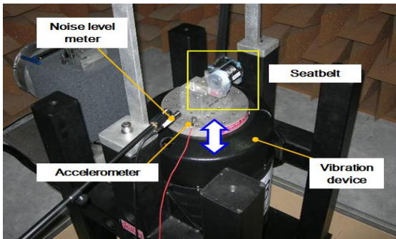
Fig. 1 Test equipment for vibration noise
