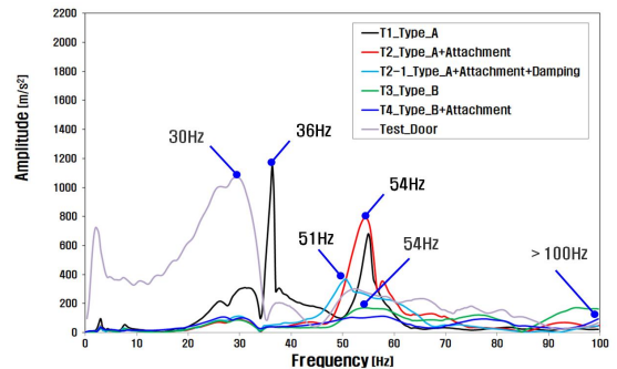
Fig. 16 Result comparison of test
