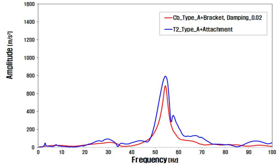
Fig. 9 Comparison of result between test and CAE
