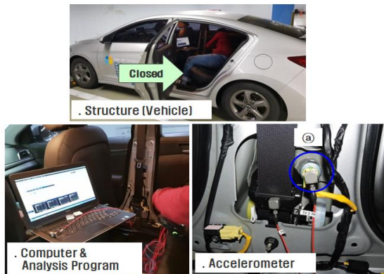
Fig. 4 Test equipment of vibration
