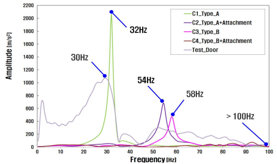
Fig. 15 Result comparison of CAE
