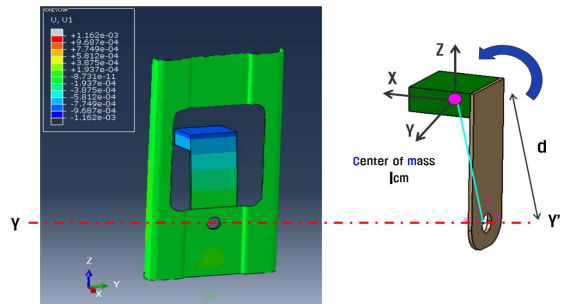
Fig. 13 Result of mode analysis
