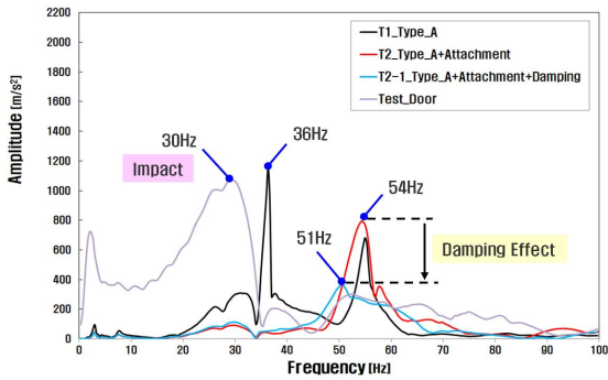
Fig. 7 Test result of type-A (frequency domain)
