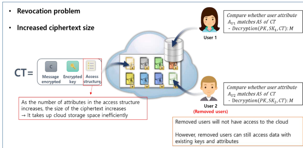
Fig. 6. Security Threats from CP-ABE
