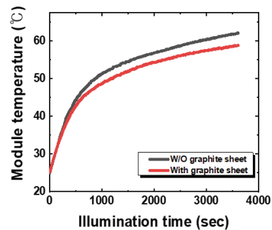
Fig. 4. Measured temperature variation of the shingled PV module without and with heat dissipation sheet as a function of the illumination time.
