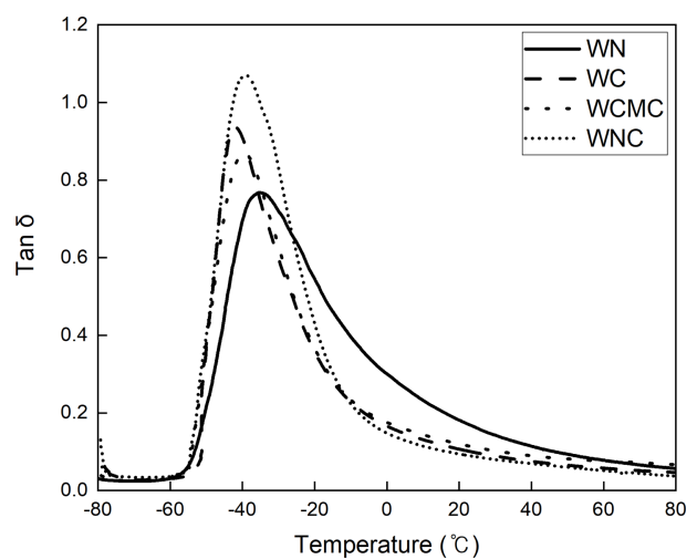
Figure 4. Tan \delta changes of the silica-SBR compounds according to types of cellulose based dispersants.
