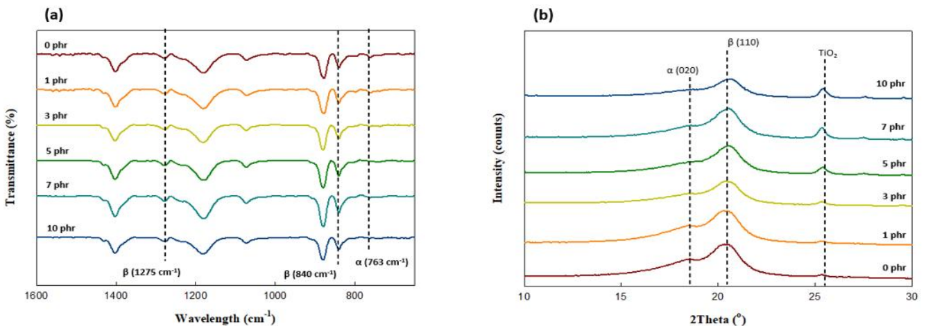
Figure 6. (a) FT-IR spectra of PVDF/ \text{TiO}_2 nano web with \text{TiO}_2 contents, (b) XRD of PVDF/ \text{TiO}_2 nano web with \text{TiO}_2 contents.
