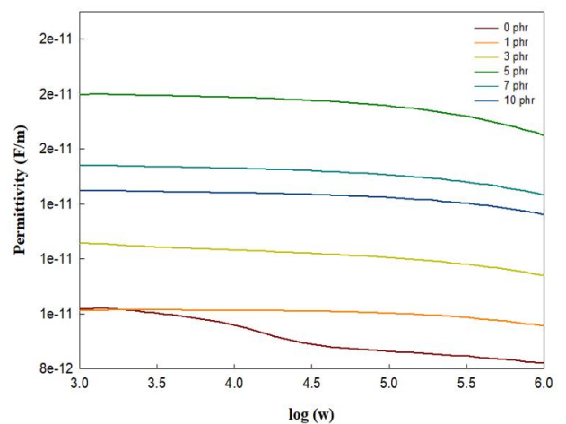
Figure 7. Dielectric constant of PVDF/TiO 2 nano web by TiO 2 components.
