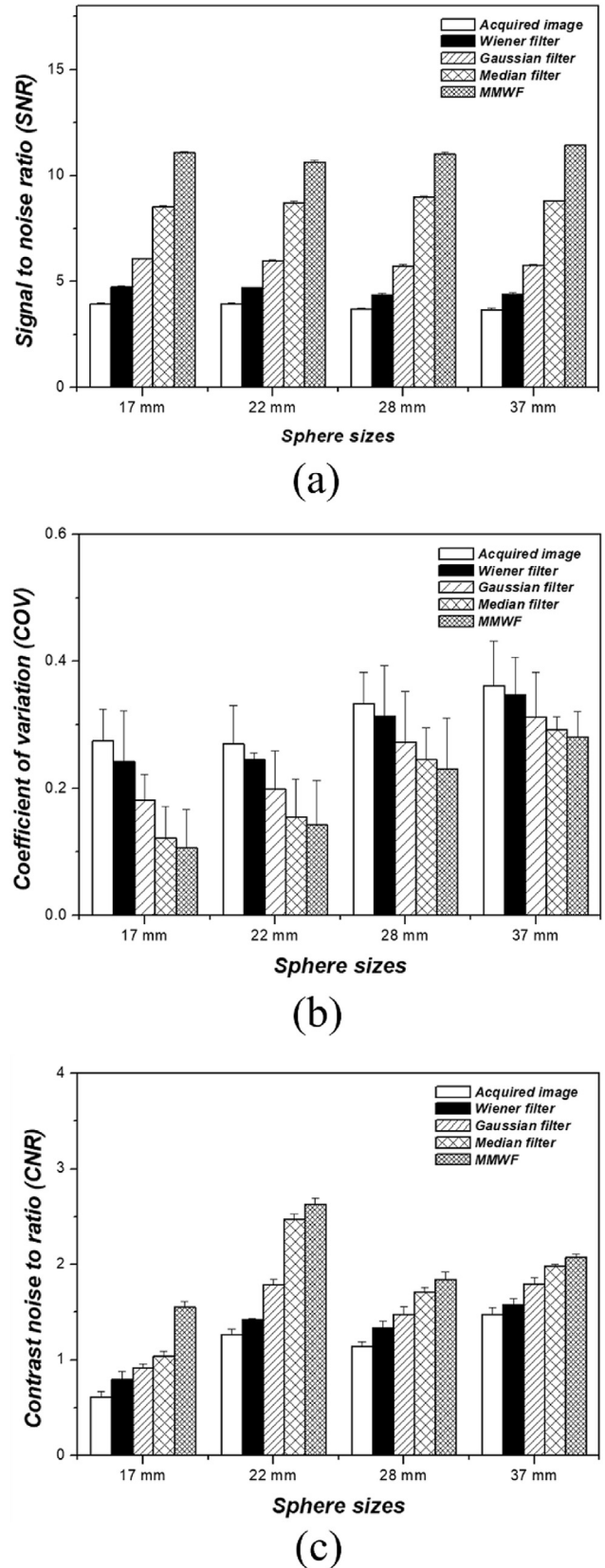
Fig. 3. Results for (a) signal to noise ratio, (b) coefficient of variation, and (c) contrast to noise ratio of the images obtained using each noise reduction filter according to sphere sizes.
