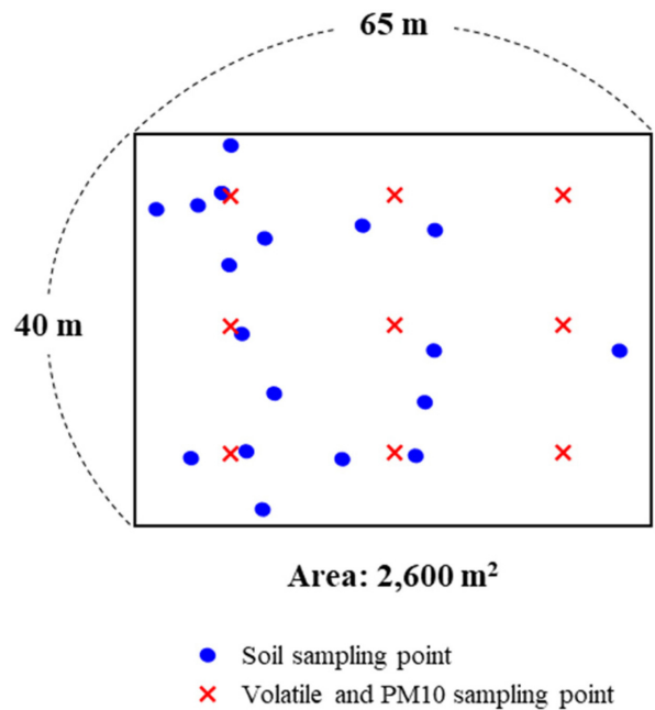
Fig. 2. Description of the target site and the sampling points for soil, volatile, and PM10.
