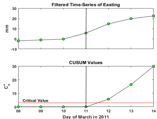
Fig. 9. Magnified the time-series and CUSUM values of KANR for seven days before and after the earthquake event (i.e., 11th March, 2011)
