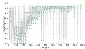
Fig. 3. Optimization Simulation History of Window Wall Ratio of Dining Room's South Facade
