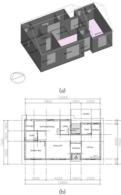
Fig. 1. Geometry of the Prototype Detached House (Nonglim-10-27-DA-1) (a) Perspective View of Design Builder Model (b) Plan of the House
