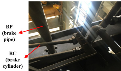
Fig. 2. Installation example of BP and BC in air brake device
