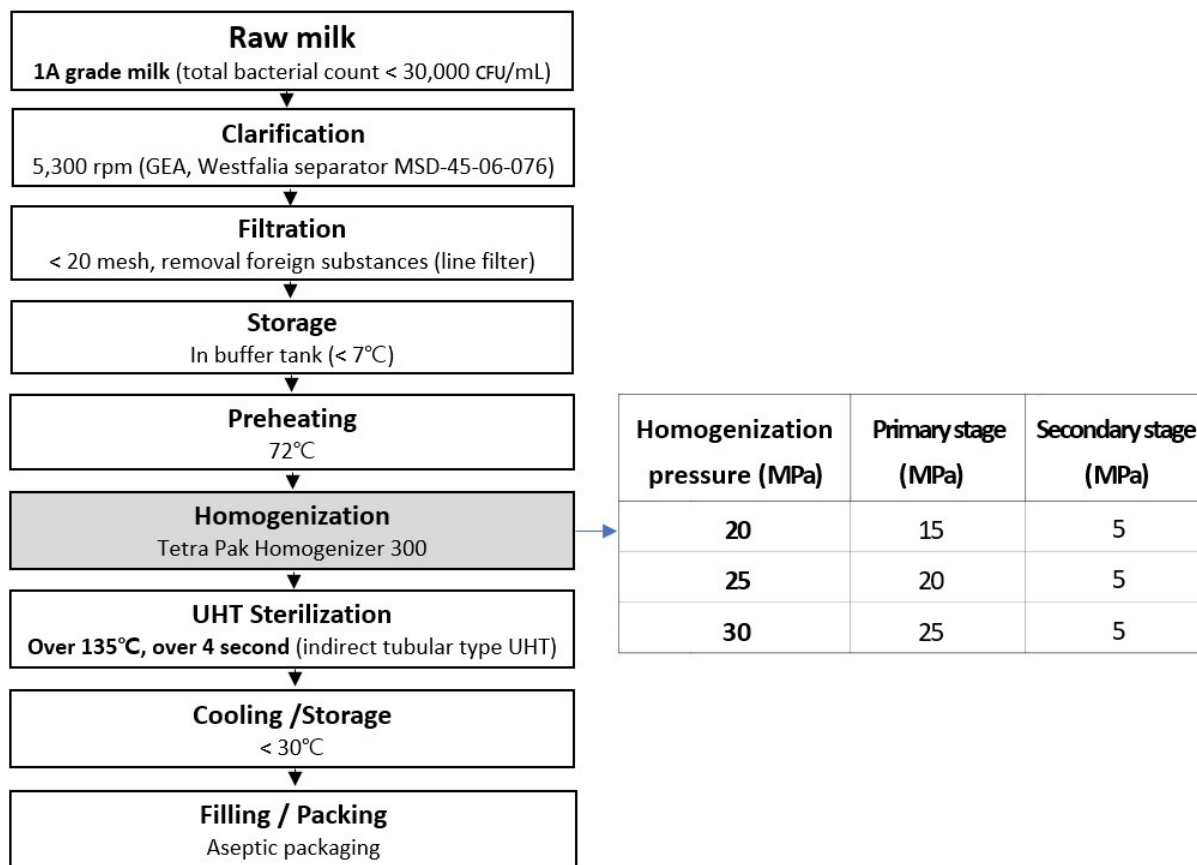
Fig. 1. Production of UHT milk at different homogenization pressures. UHT, ultra high temperature.
