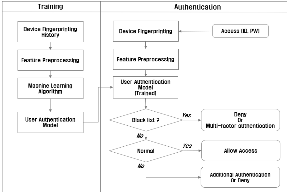
Fig. 3. User Authentication Model Based on Device Fingerprinting Using Machine Learning
