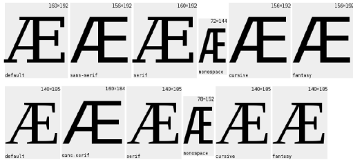
Fig. 2. Rendering Results of U+00C6 by Browser (Upper : Firefox24, Lower : Chromium35)
